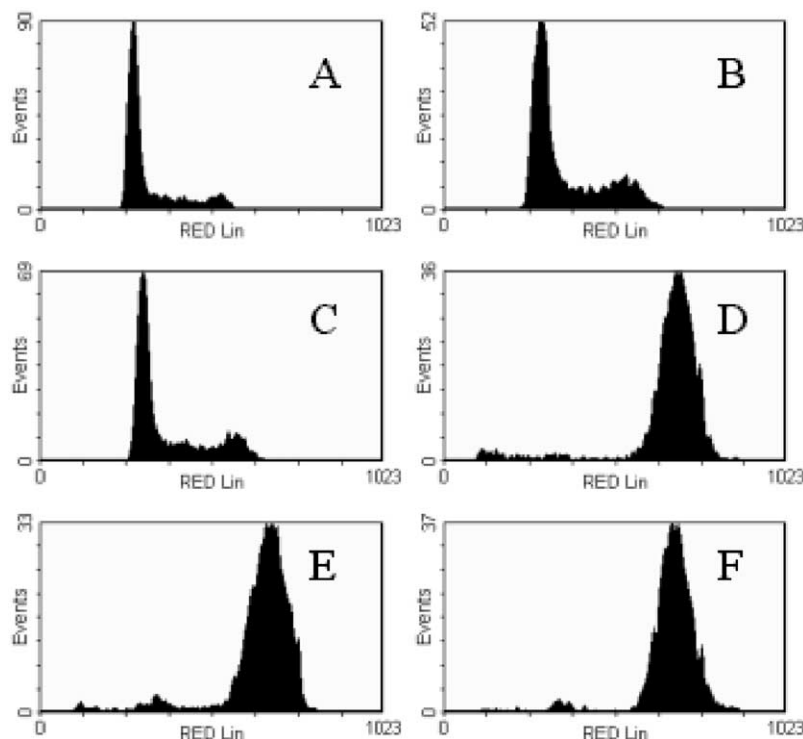
Figure 2. DNA profiles of cells treated for 24 h with compound 3c : A, control cells; B, 3c 10^{-8} M; C, 3c 10^{-7} M; D, 3c 10^{-6} M; E, 3c 10^{-5} M. F, cell treated with 3c 10^{-5} M for 48 h.
