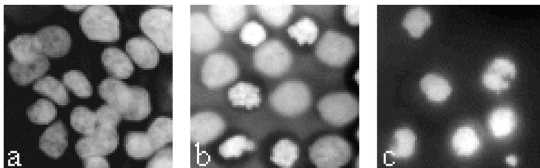
Figure 4. Photographs of control cells (a), cells treated with 3c 10^{-5} M for 24 h (b) and 48 h (c). Cells were stained by Hoechst 33342 as reported in Section 5.
